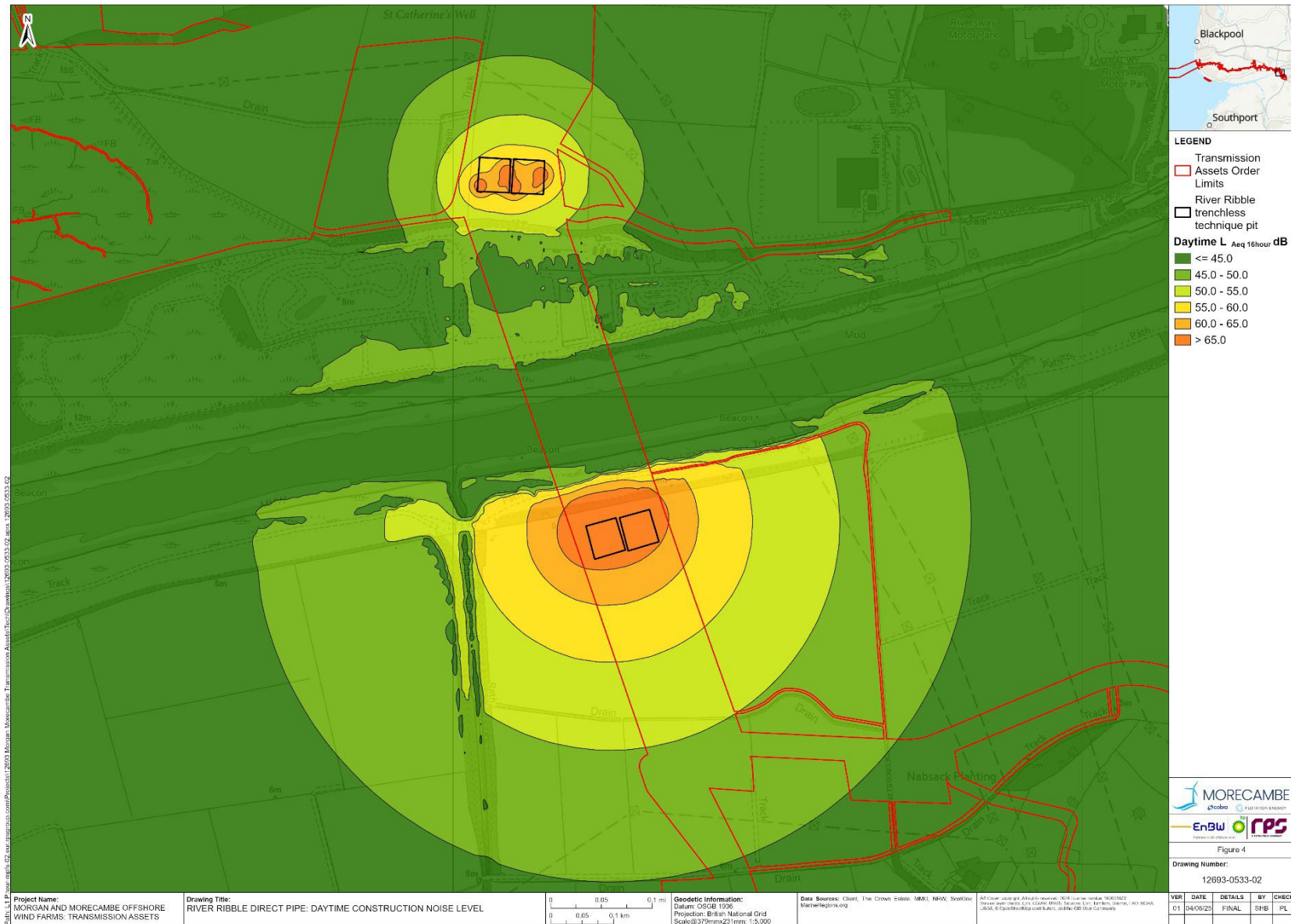
Figure 4: Noise modelling for the River Ribble direct pipe method (daytime)
